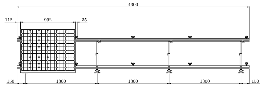
VISTA FRONTAL
